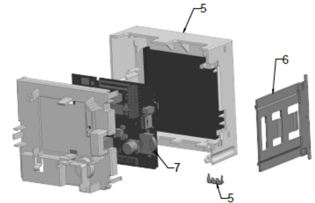
Displayunit without Display
