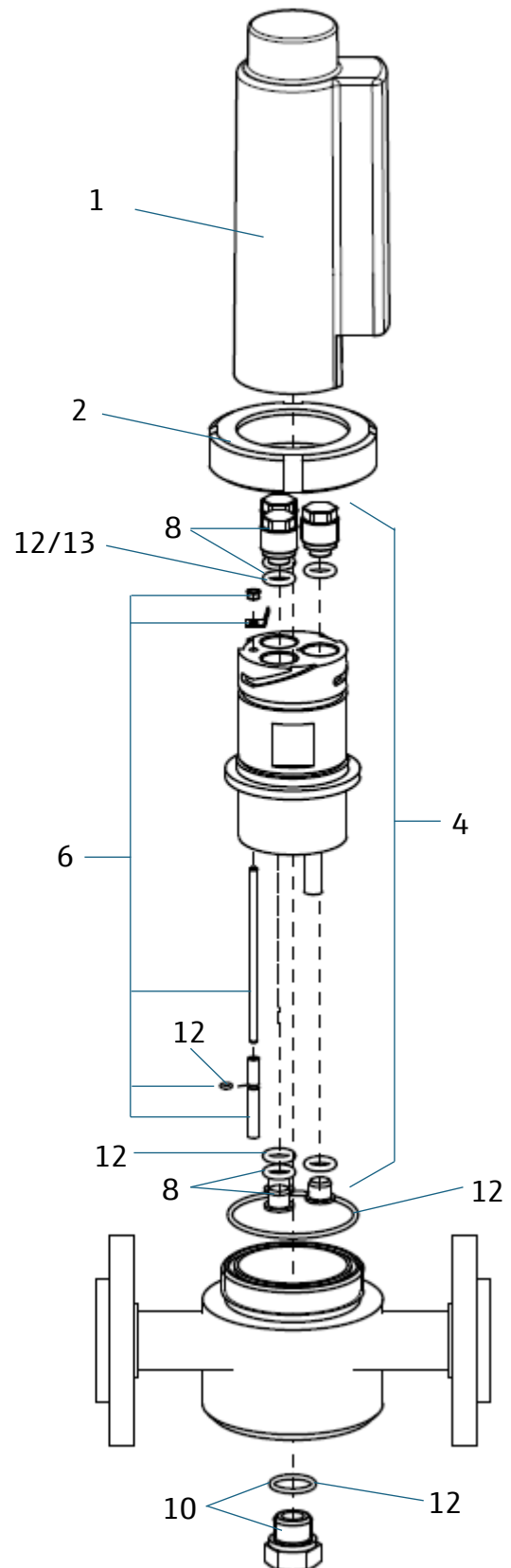
CPA240-2++++++ PVDF version
