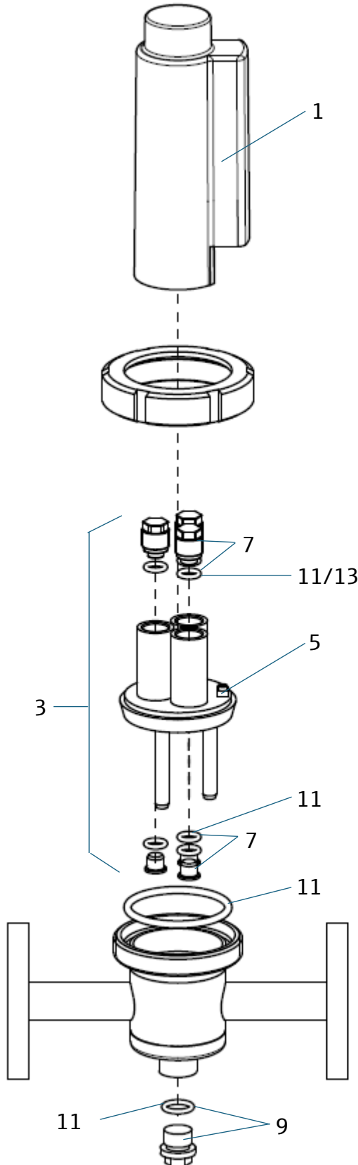
CPA240-3++++++ Stainless steel version
